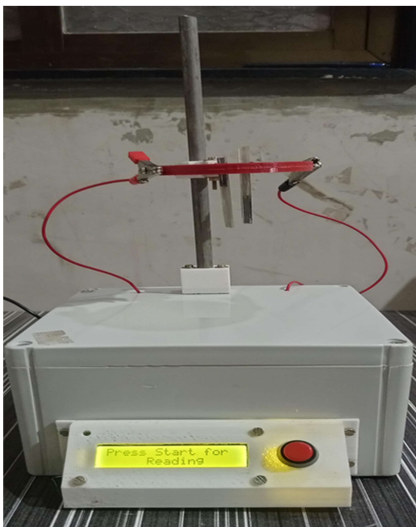
Developed-Potentiometric system for bio medical applications
